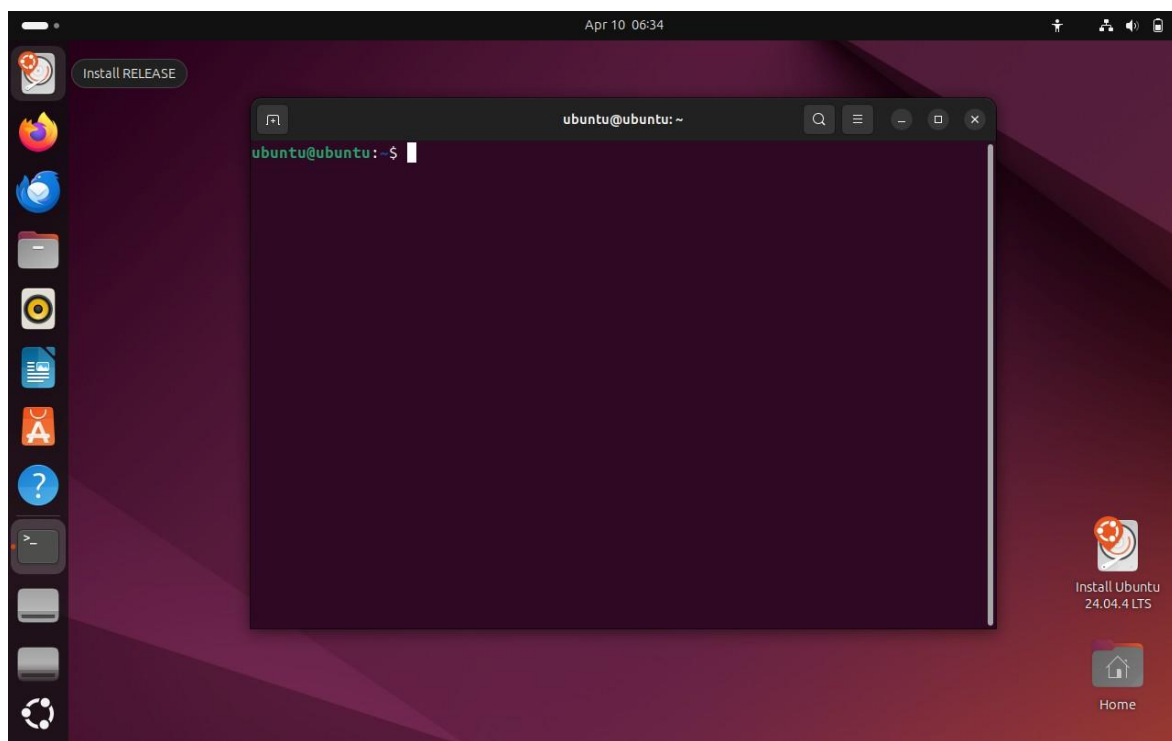
Fig 1.4: Ubuntu Terminal
