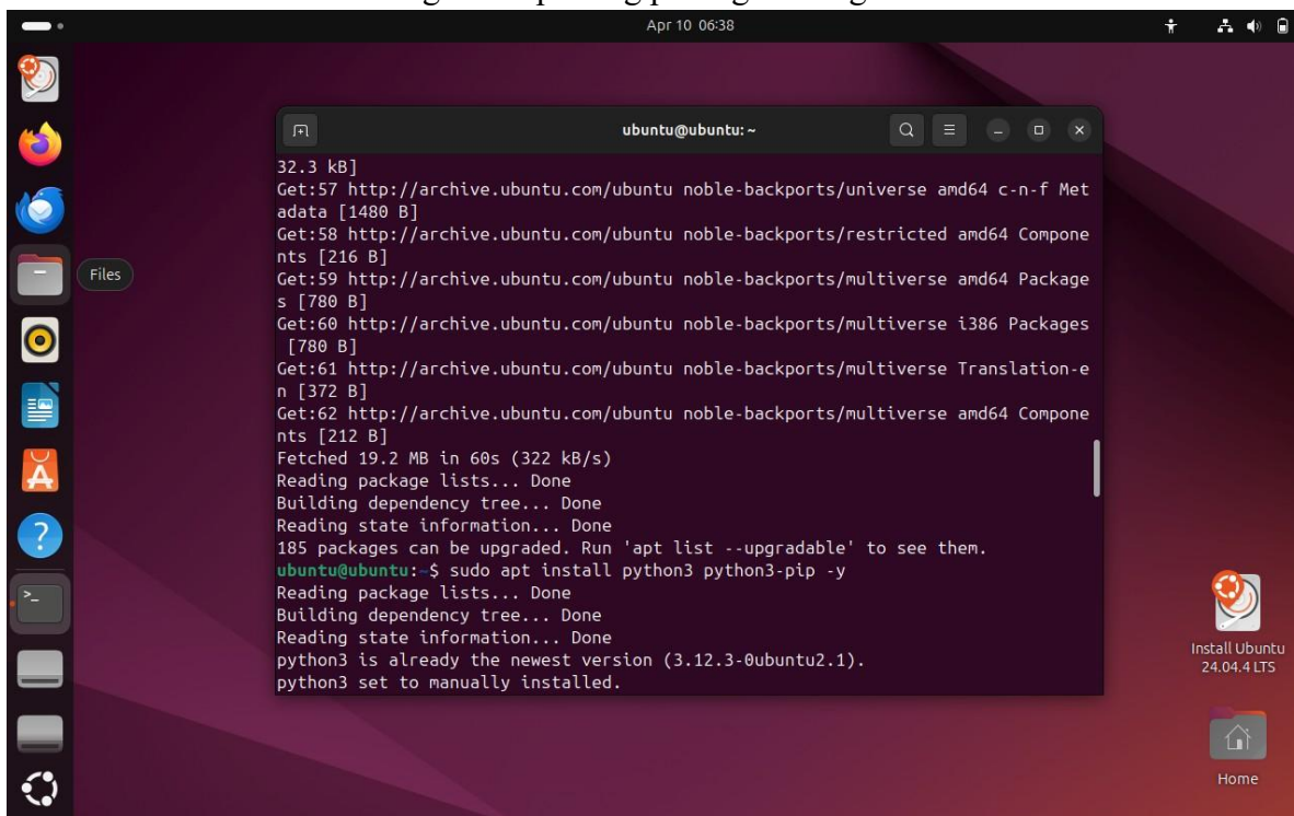
Fig 1.6: Installing python
